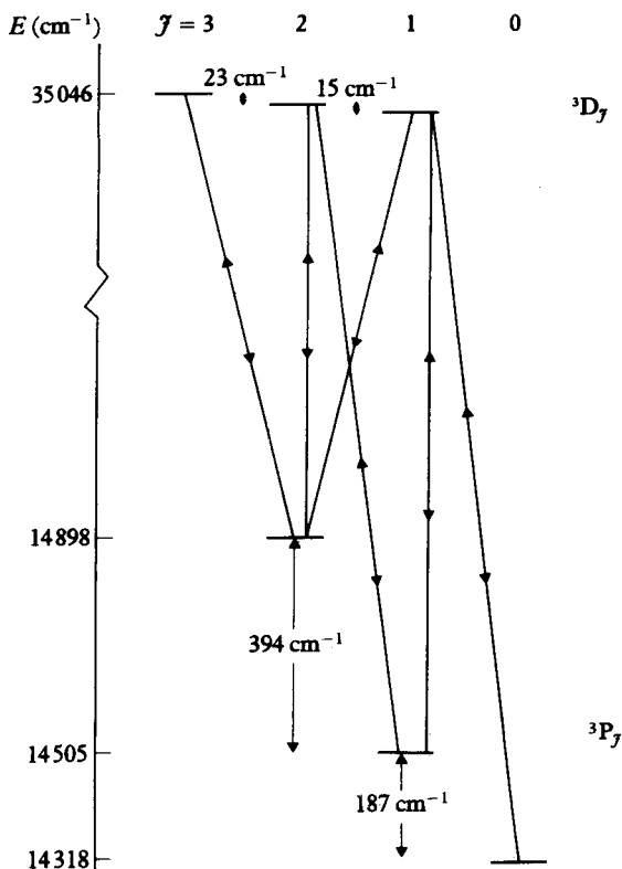
8.4 The transitions between the (5s5d) {}^3D_7 and the (5s5p) {}^3P_7 terms of strontium. The left-hand side shows the energies above the (5s^2) {}^1S_0 ground state in \text{cm}^{-1} .
